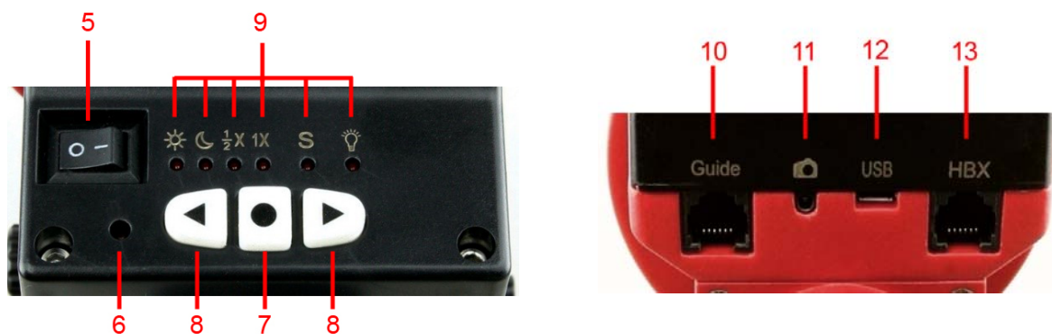
Figure 5. Control panel and ports of a SkyGuider™ Pro mount head
