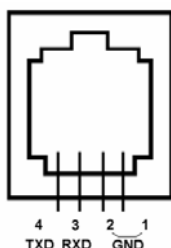
Figure 27. Serial port pin out on an 8408 hand controller
